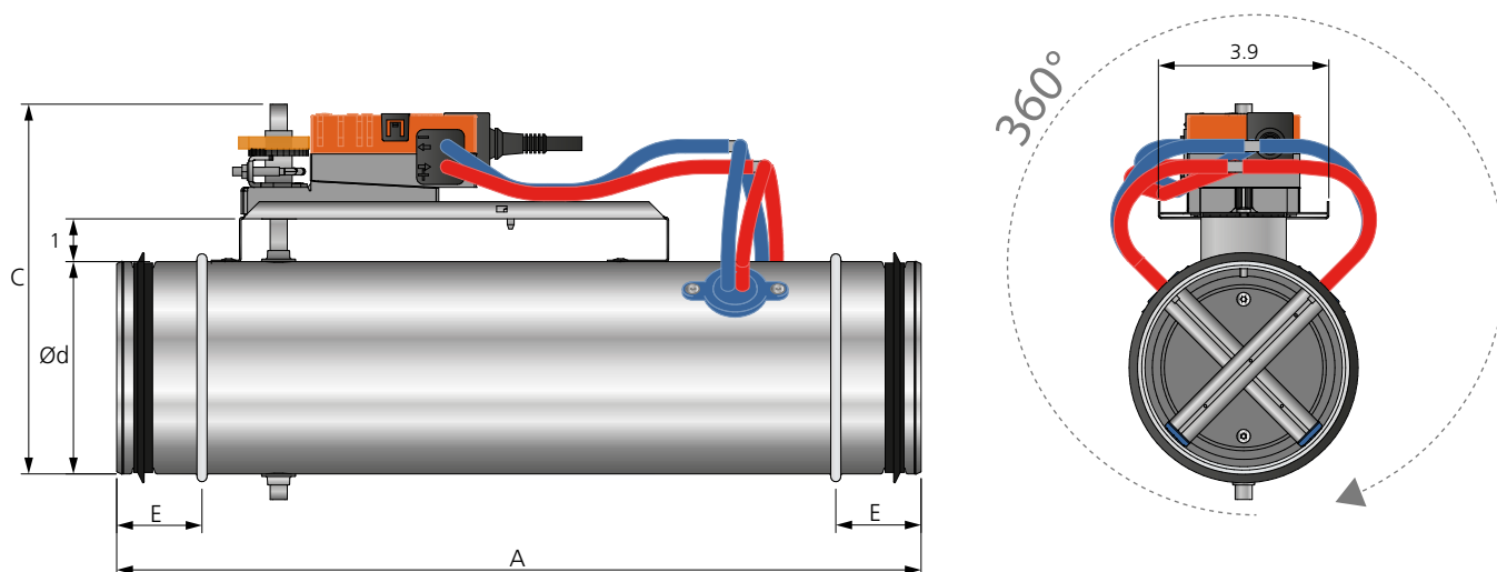
Figure 3. Dimensions (in), REACT V BBAC circular. The damper can be installed at an optional angle.
