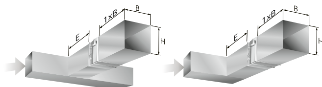
Figure 9. Straight duct section requirements in rectangular ducts.
