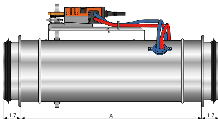
Figure 4. Dimensions with DUCT ADAPTER installed (in), REACT V BBAC circular.
