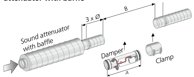
Figure 6. Straight duct section requirements 3 \times \varnothing in case of sound attenuator with baffle or centre body.
