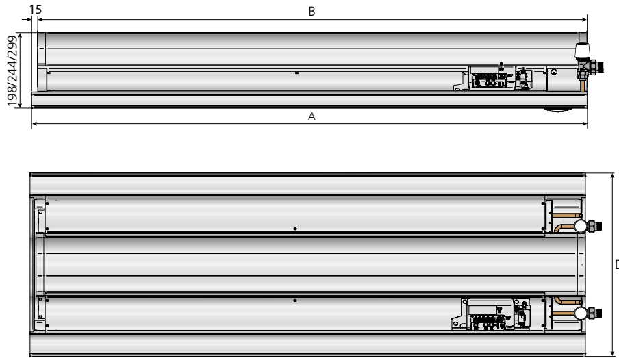
Figure 13. Dimension sketch - full size
