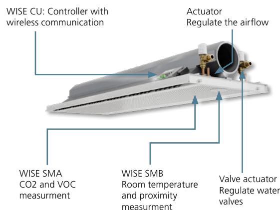
Figure 15. Factory fitted components
