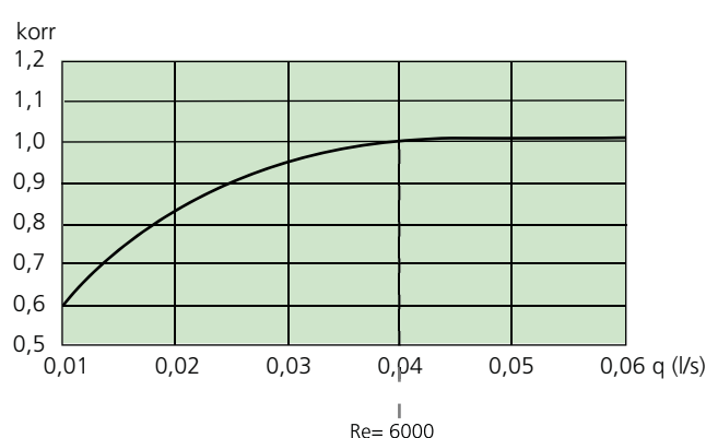
Diagram 2. Water flow – capacity correction, heating
