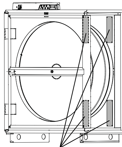
Cover plates for pipe lead-through. Two cover plates are removed, either in the lower level or the upper level, depending on the variant.
